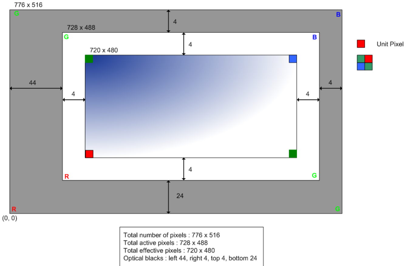
Figure 3-1 Pixel Array Structure
