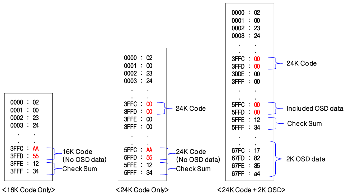
Figure 7-1 EEPROM Boot Sequence
