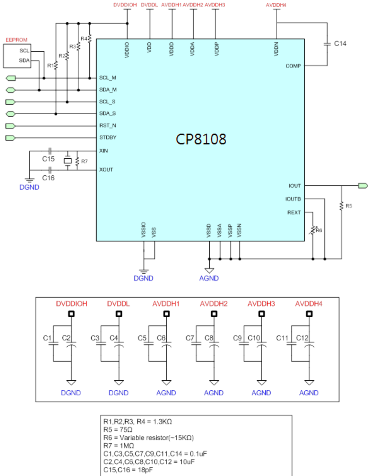
Figure 15-1 Typical Circuit Configuration(Analog)
