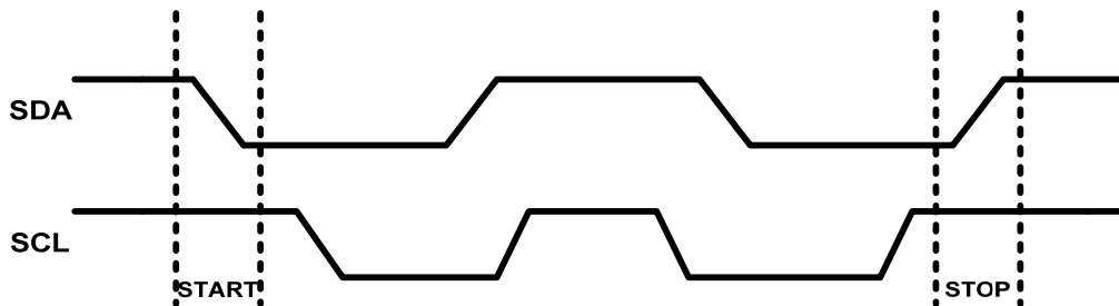
Figure 5-3 Start / Stop
