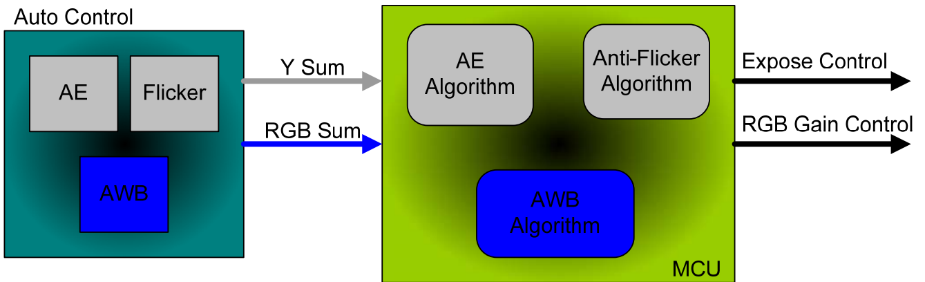
Figure 10-34 Auto Control Function
