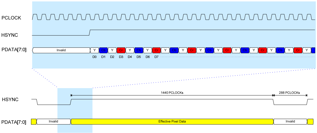
Figure 4-1 Horizontal Timing
