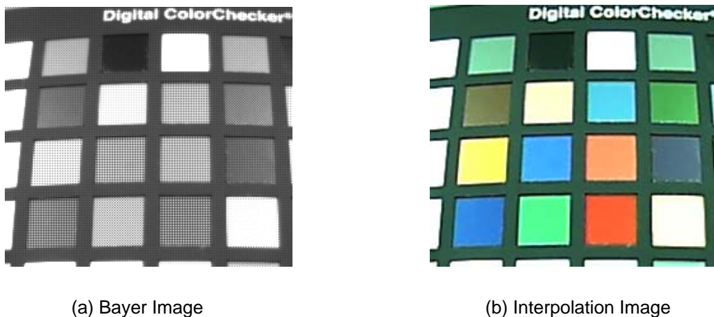
Figure 10-10 Color Interpolation Image
