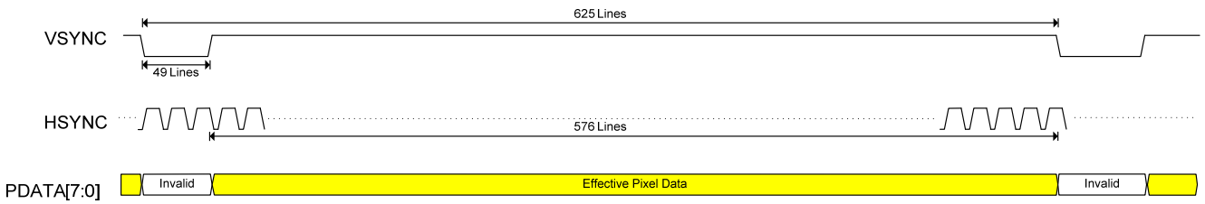
Figure 4-2 Vertical Timing
