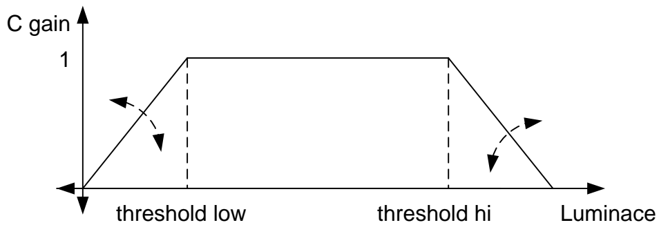
Figure 10-25 Applying Gain on Luminance Threshold
