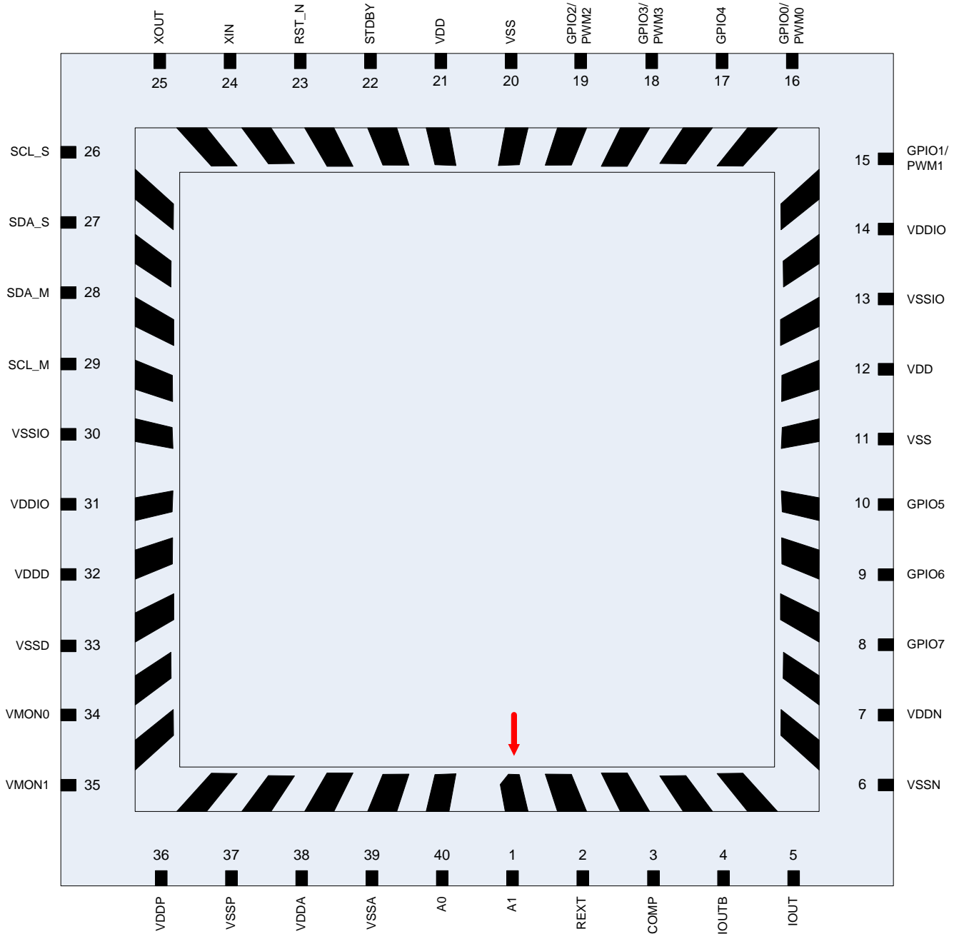
Figure 14-1 40 Pin CLCC PKG Pin Map(Analog)
