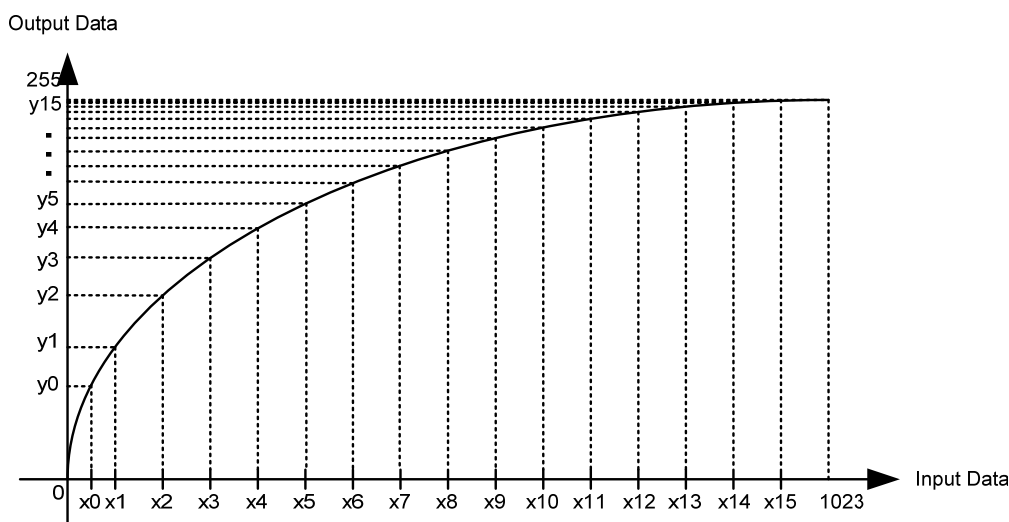
Figure 10-14 GAMMA register and GAMMA value
