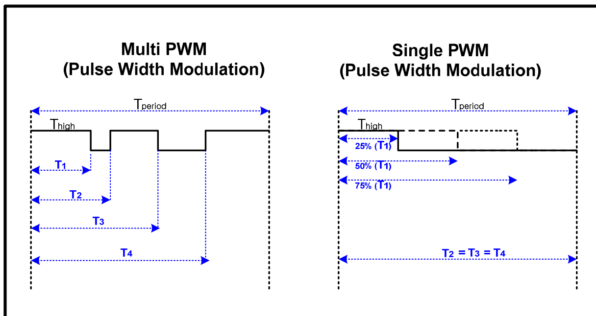
Figure 5-8 PWM Generation
